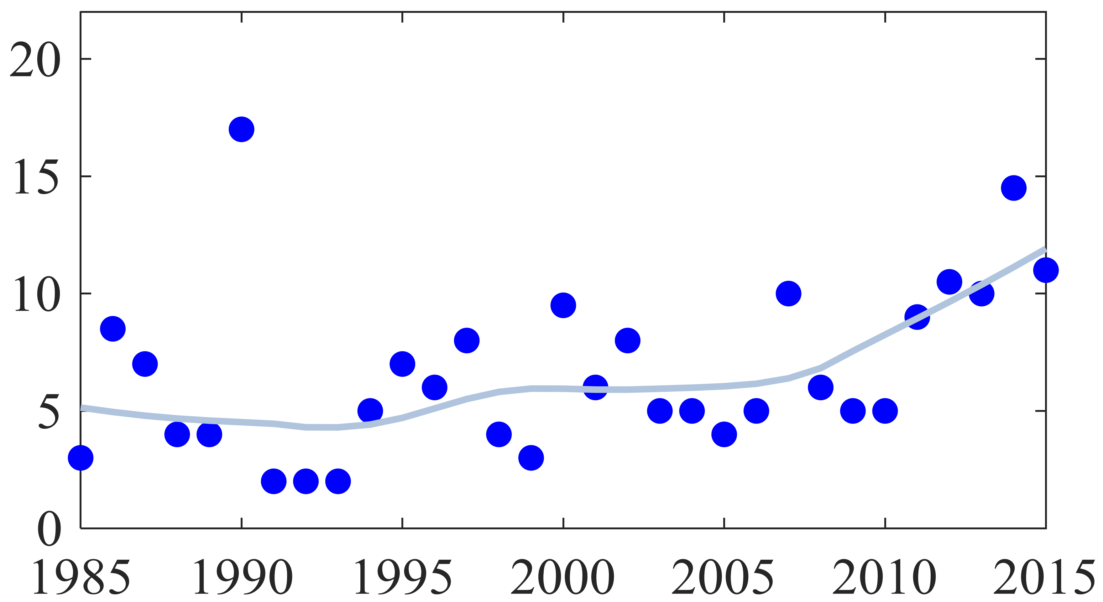
Subtropics (S)
