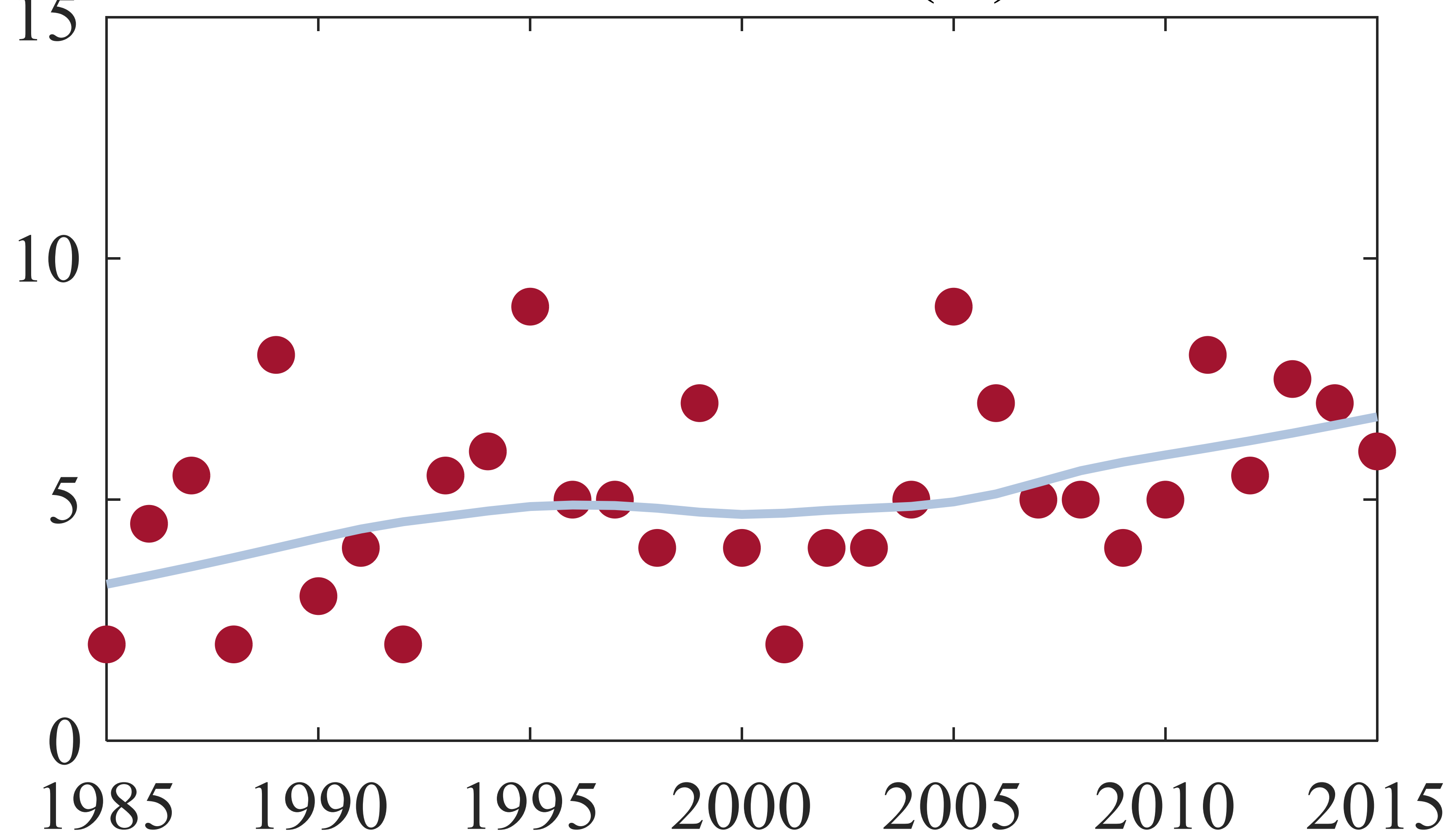
Midlatitudes (S)
