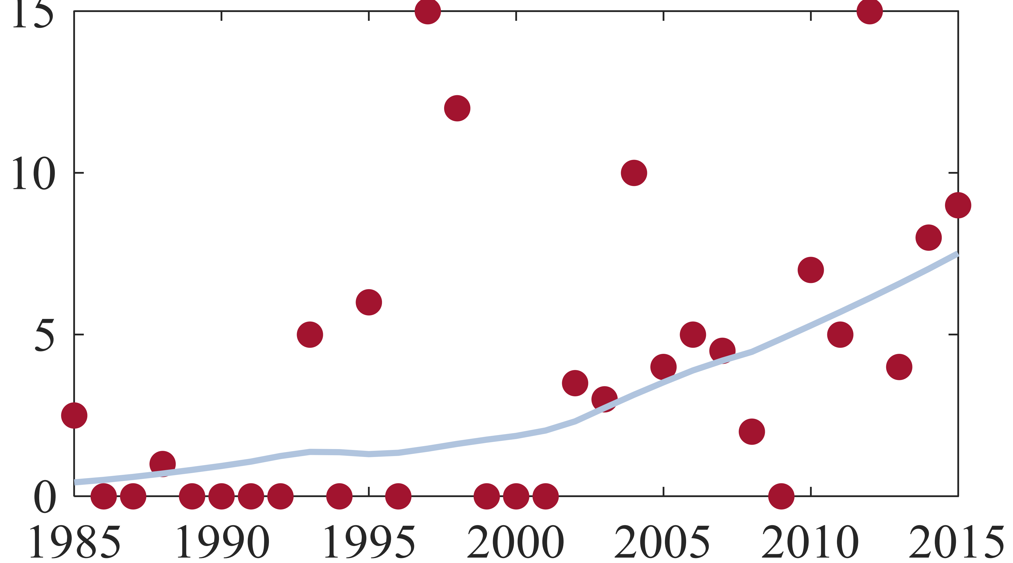
Midlatitudes (S)
