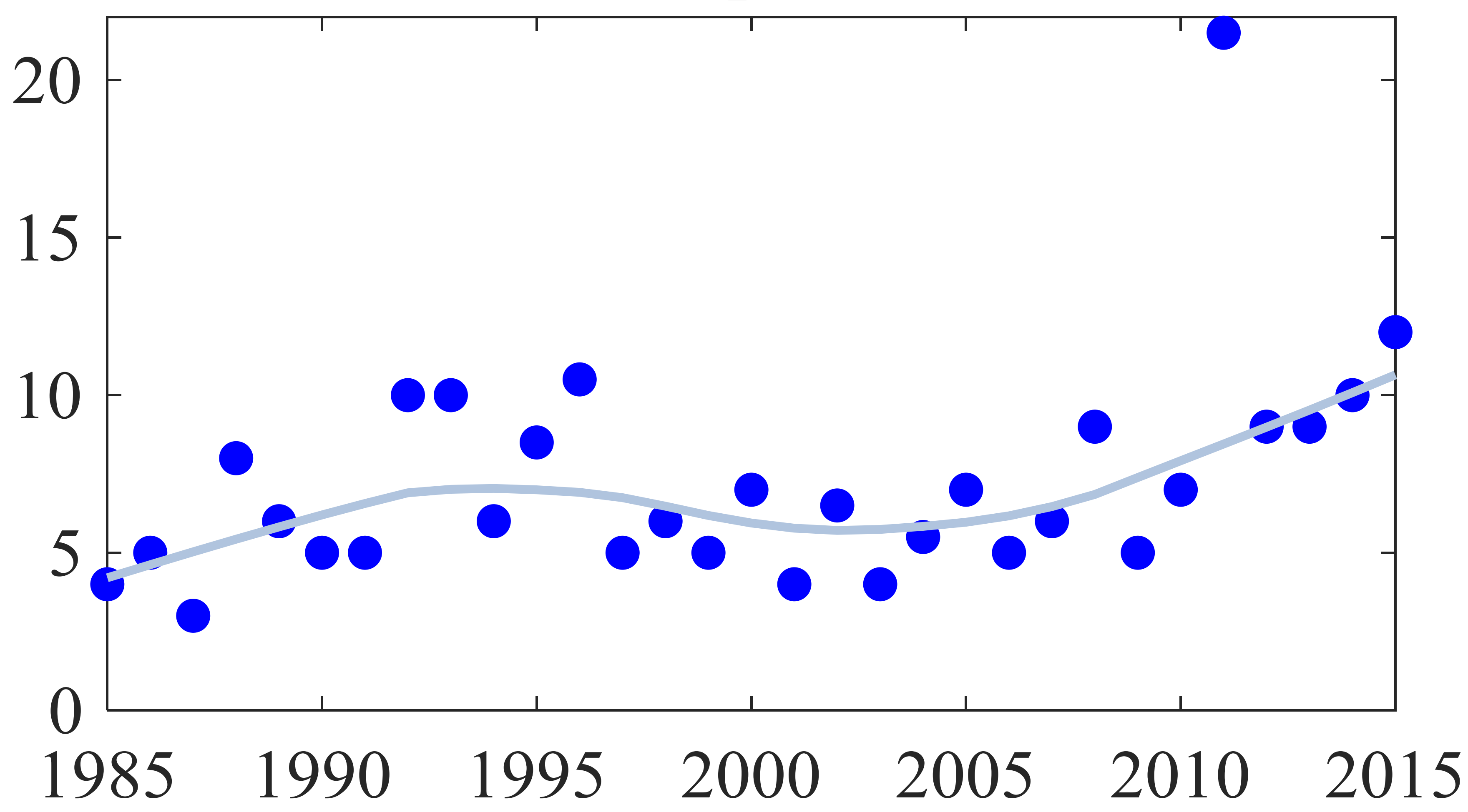
Subtropics (N)
