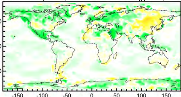
Northward wind (850 hPa) link to northward OGW drag (30 hPa)
