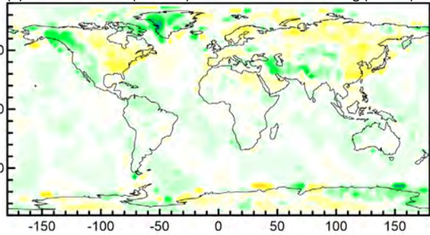
(c) Eastward OGW drag (30 hPa): fraction of variance explained
