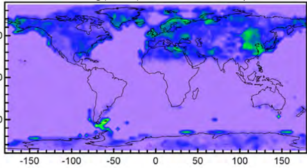
Northward OGW drag (30 hPa): fraction of variance explained
