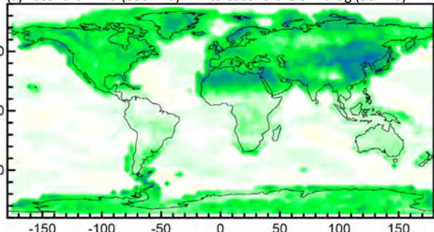
(b) Northward wind (850 hPa) link to eastward OGW drag (30 hPa)
