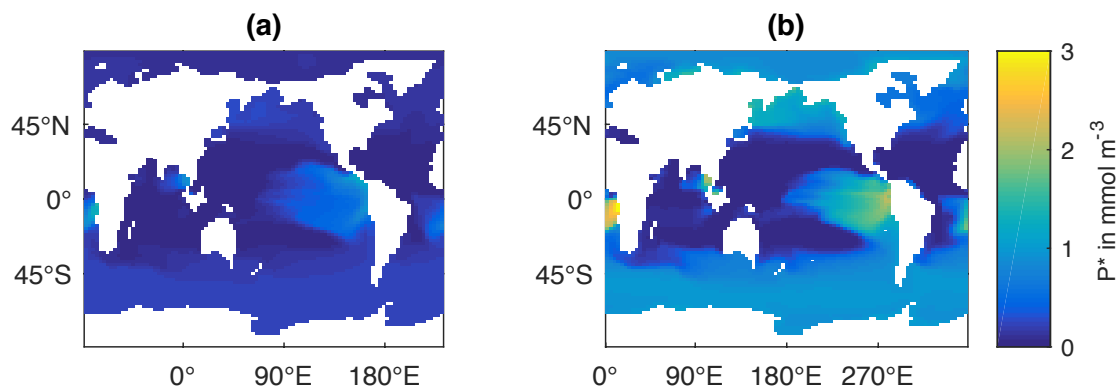
Fig. S2: Spatial distribution of P^*=P-N/16 (dissolved P, N) in the surface ocean for (a) the preindustrial case and (b) simulation year 5000 for Weath0.15 .
